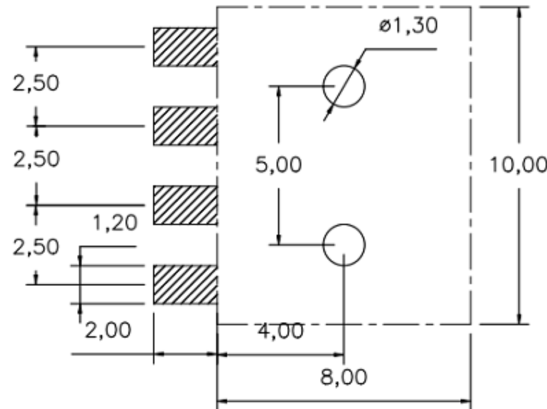
RECOMMENDED PCB LAYOUT TOP VIEW (.XX±0.05)
